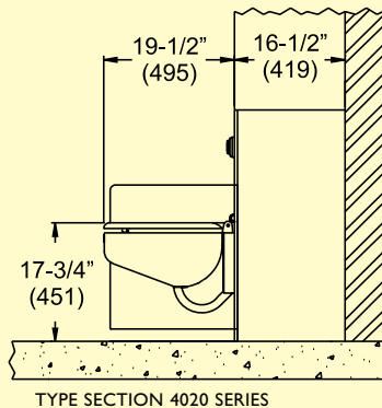
4026 BUILT-IN BACK WALL WASTE OUTLET 4027 BUILT-IN SIDE WALL WASTE OUTLET 4028 BUILT-IN FLOOR WASTE OUTLET
